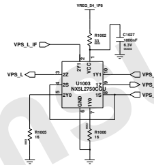
Audio Switch
