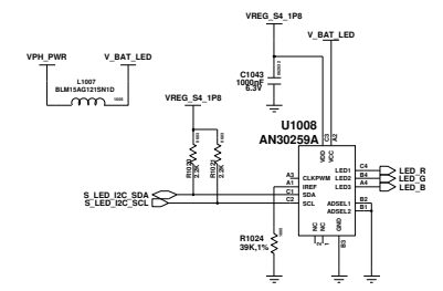
SVC LED DRIVER
