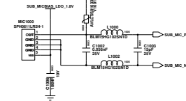
2nd MIC
