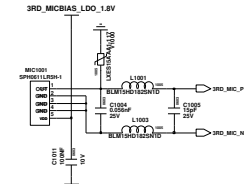
3rd MIC
