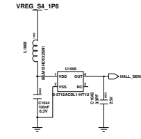
HALL SENSOR
