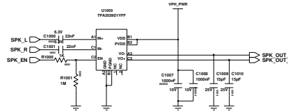
SPK AUDIO AMP
