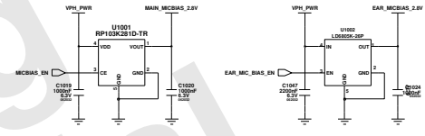
MIC Bias LDOs
