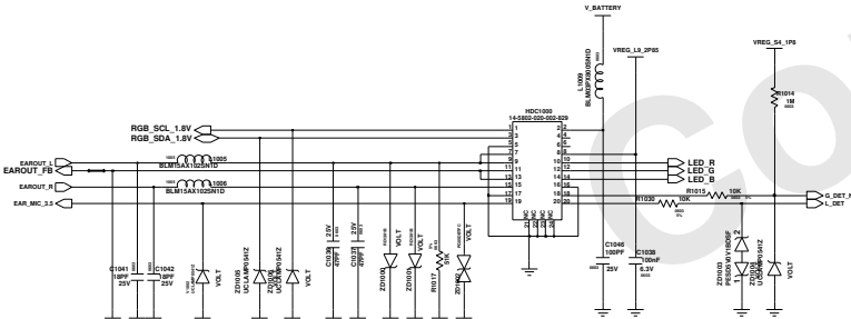
RCV + E/J + SVC LED
